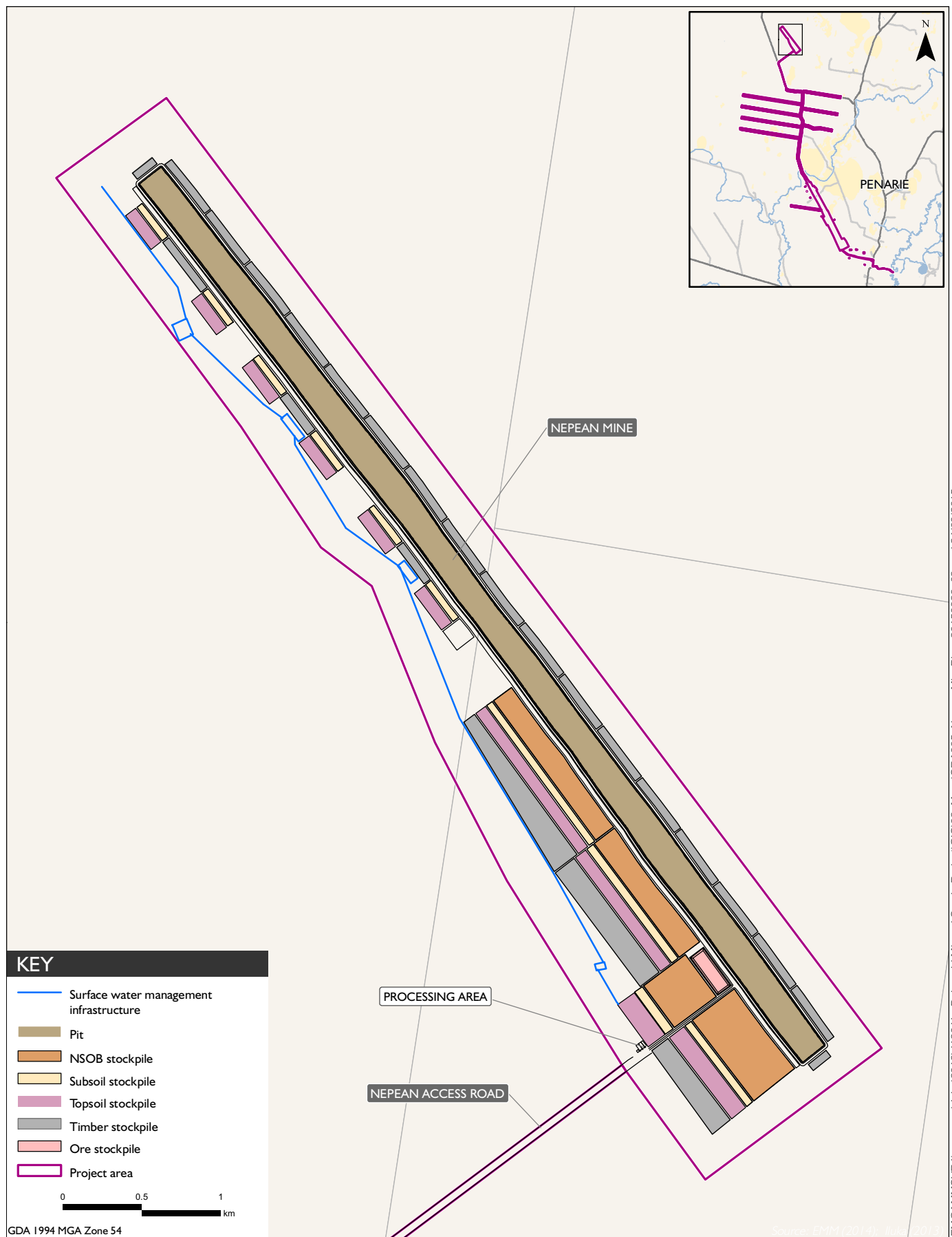
Nepean indicative mine layout
