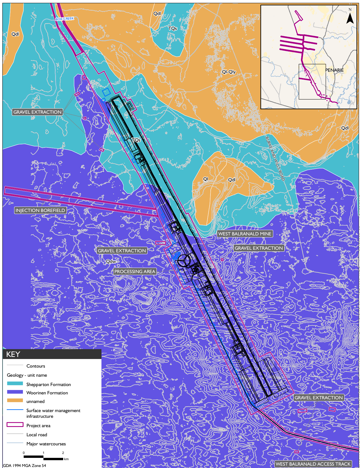
Geology and topography of the West Balranald project area
