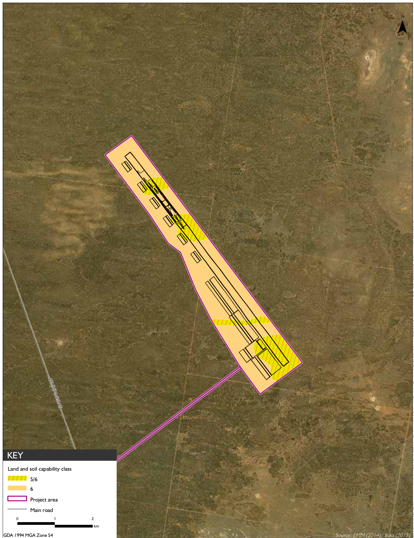
Pre-mining land and soil capability in the Nepean project area
