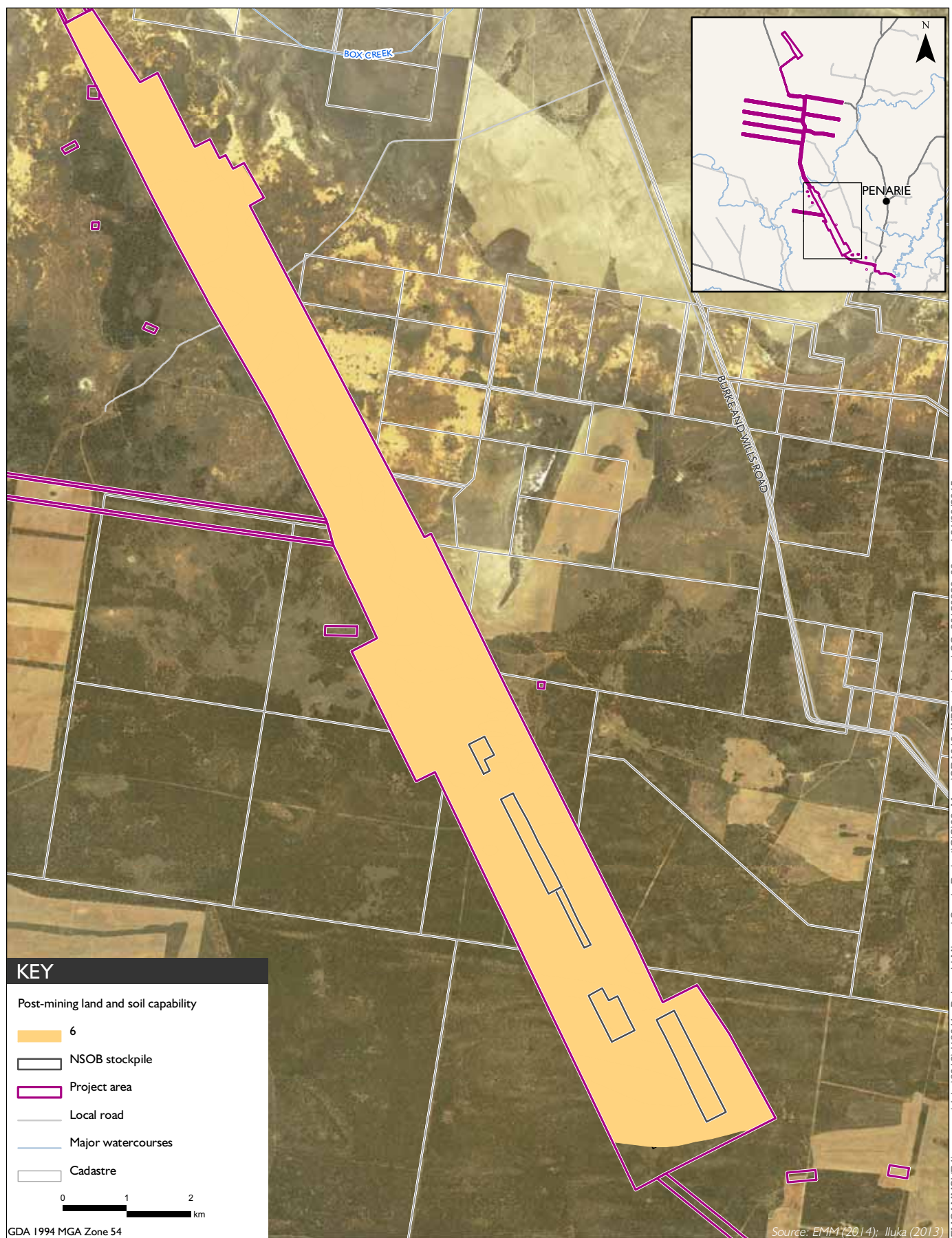
Post mining land and soil capability for West Balranald
