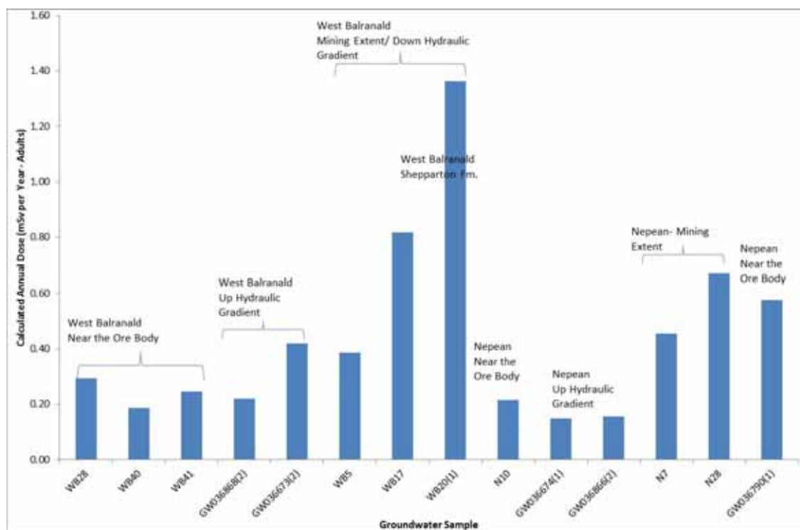
Figure 5-1 – Calculated Annual Dose of Waters per Zone
