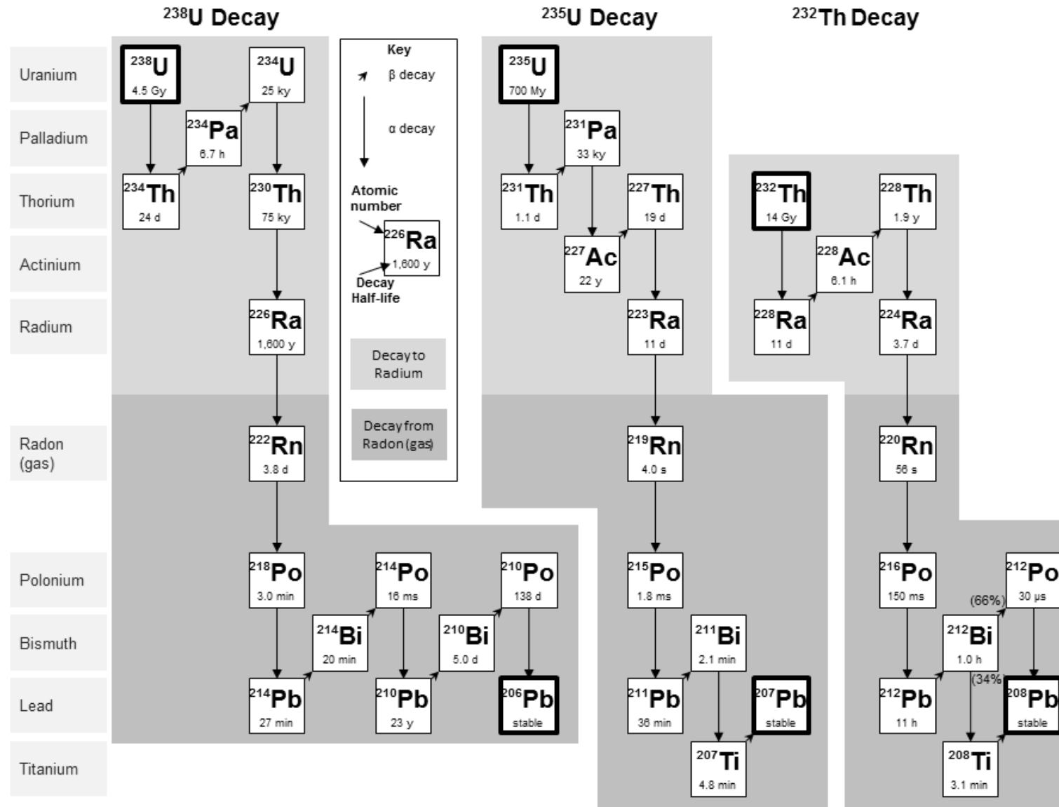
Figure 5: Radionuclide decay chains U-238, U-235 and Th-232.
