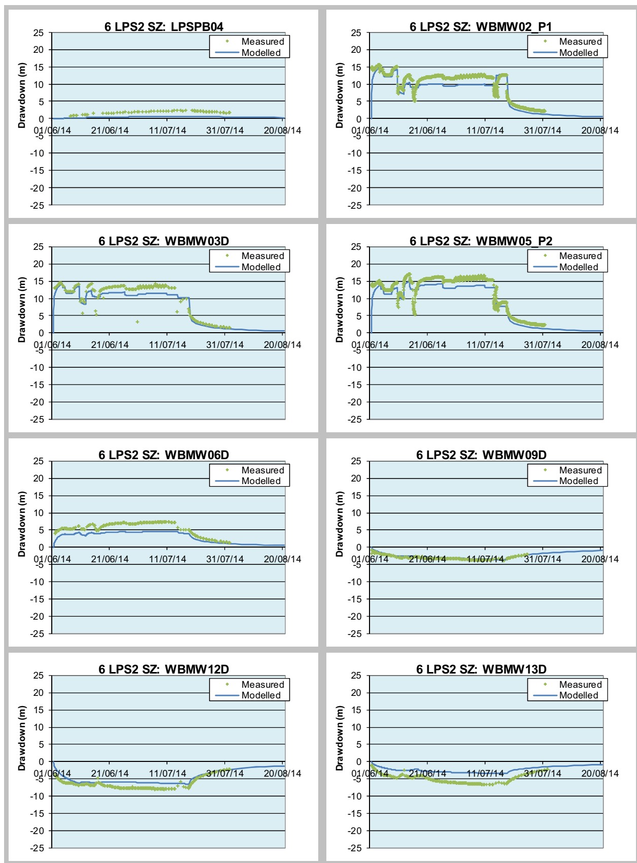
Figure 4.9 : LTT measured and modelled hydrographs
