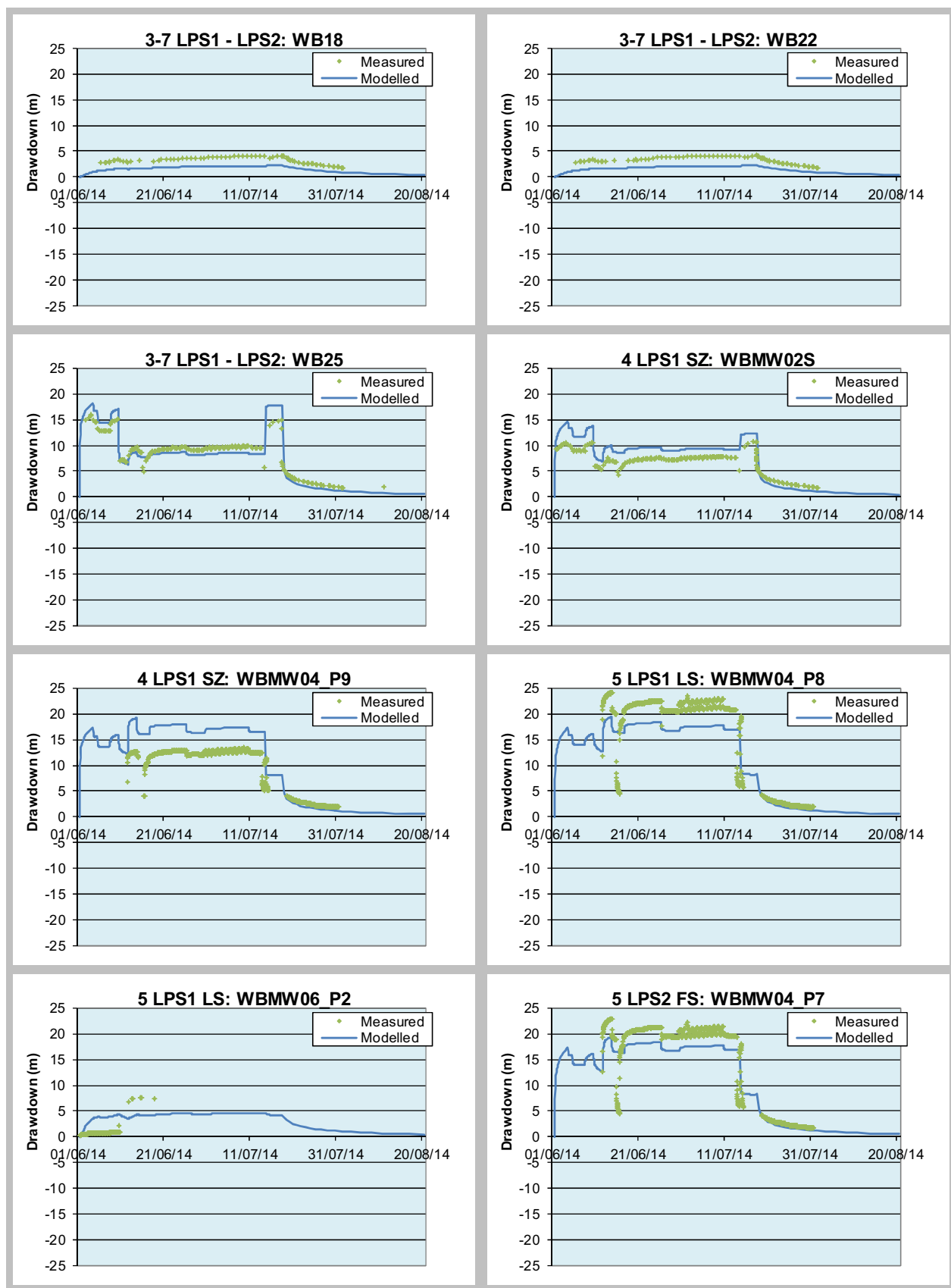
Figure 4.8 : LTT measured and modelled hydrographs
