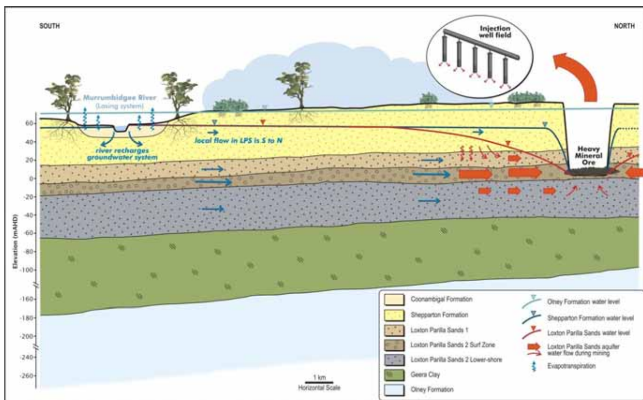
Figure 2.29 : Conceptual hydrogeology from the Murrumbidgee River to the southern end of the West Balranald deposit, during mining
