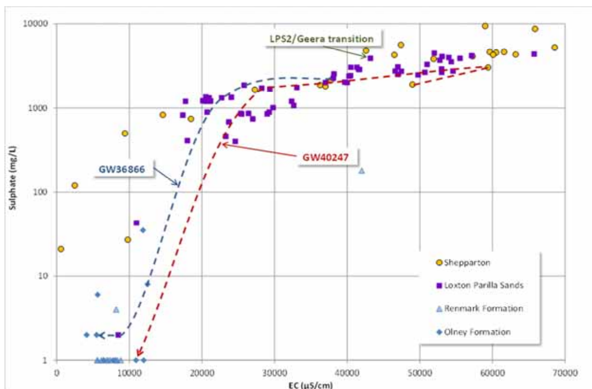
Figure 2.24 : Salinity and sulphate relationships for all bores
