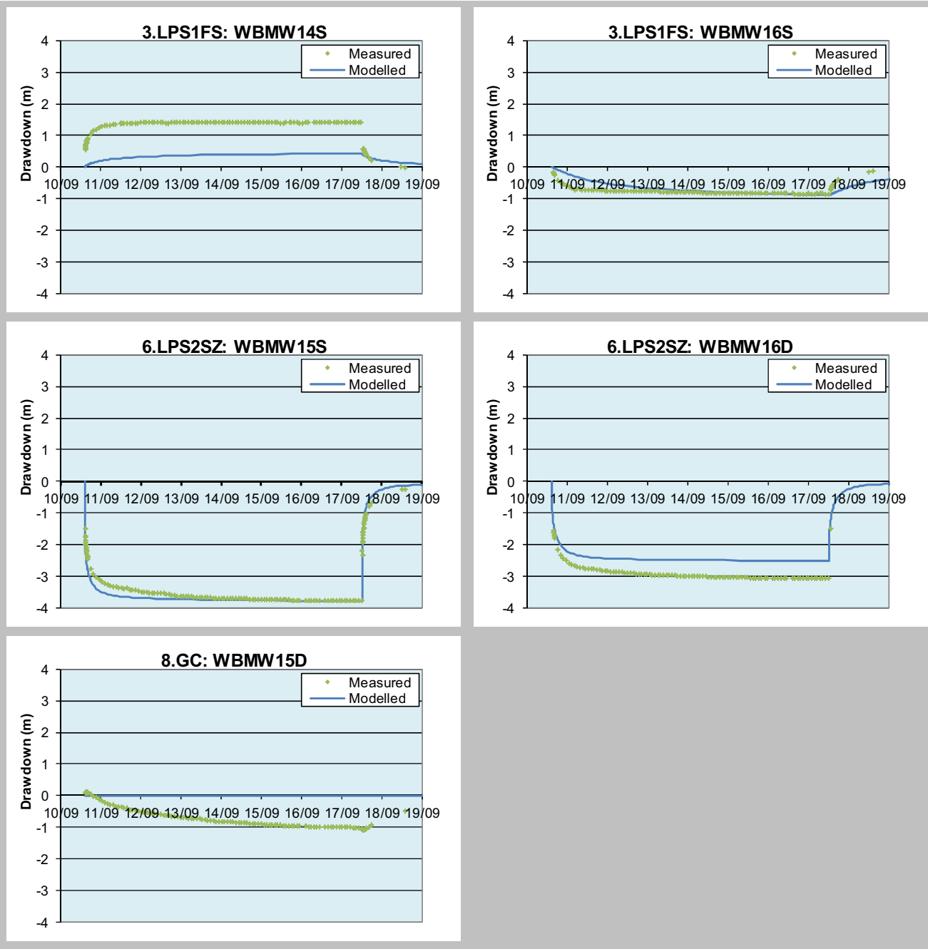
Figure 4.27 : “Upson Downs” measured and modelled hydrographs
