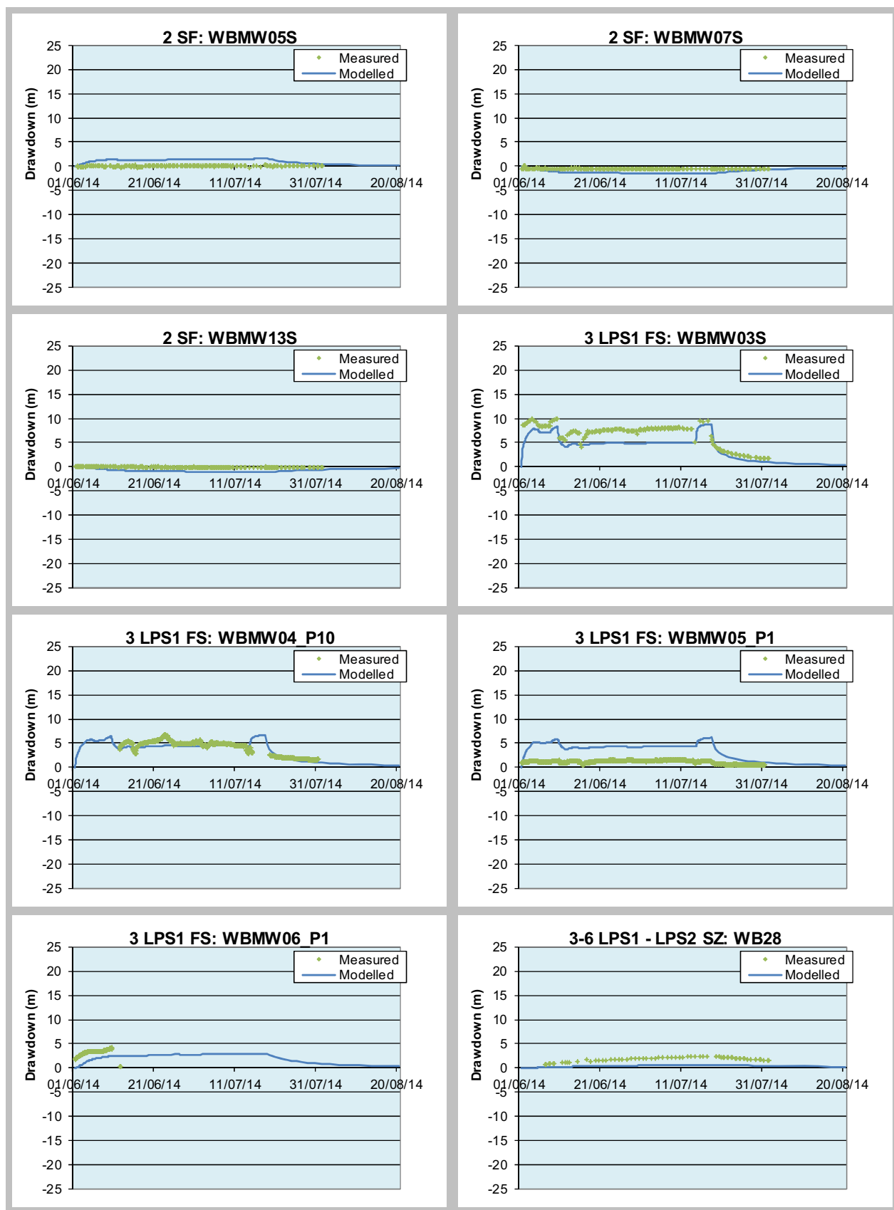
Figure 4.7 : LTT measured and modelled hydrographs
