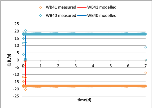
Figure 4.17 : TN5 measured and modelled production and injection
