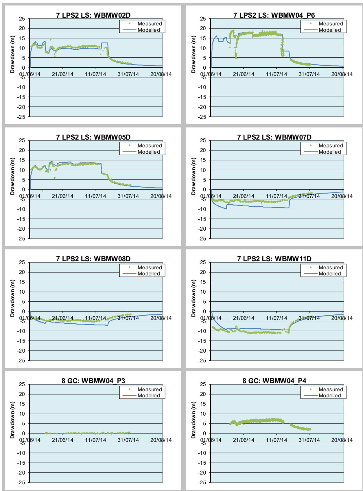
Figure 4.10 : LTT measured and modelled hydrographs
