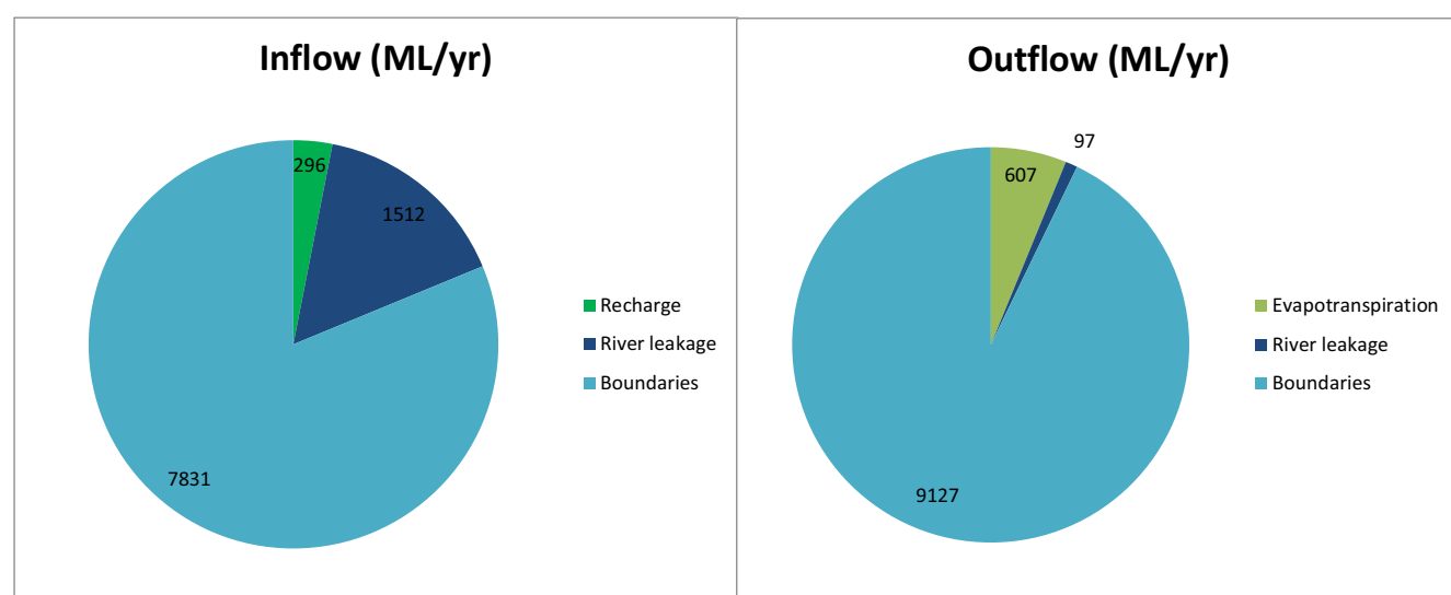
Figure 4.43 : Modelled pre-development steady state water balance
