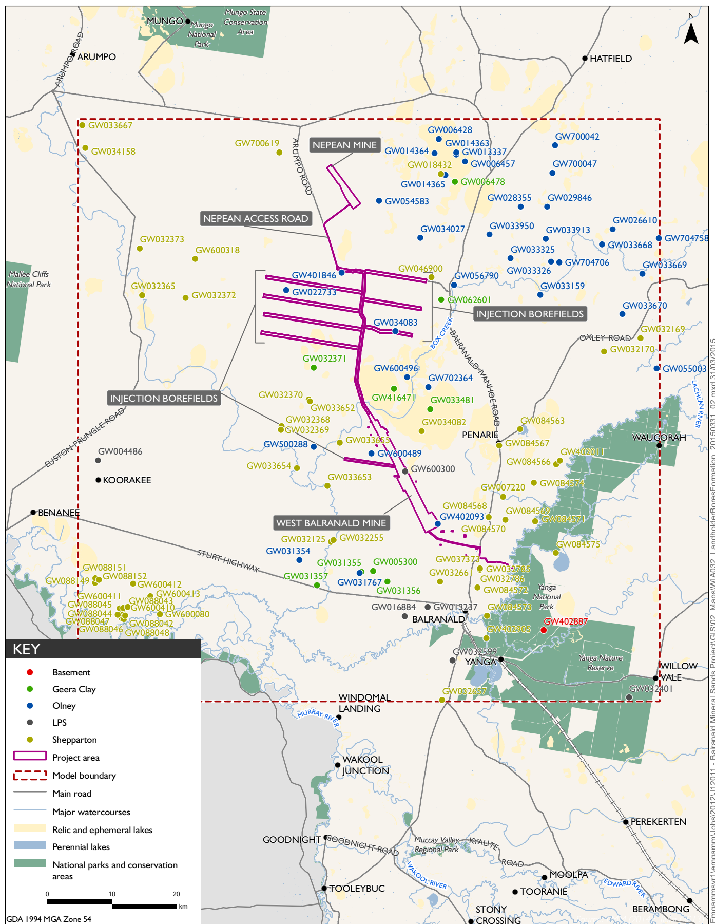
Landholder bores and formation screened Balranald Mineral Sands Project Water Assessment Figure 6.8
