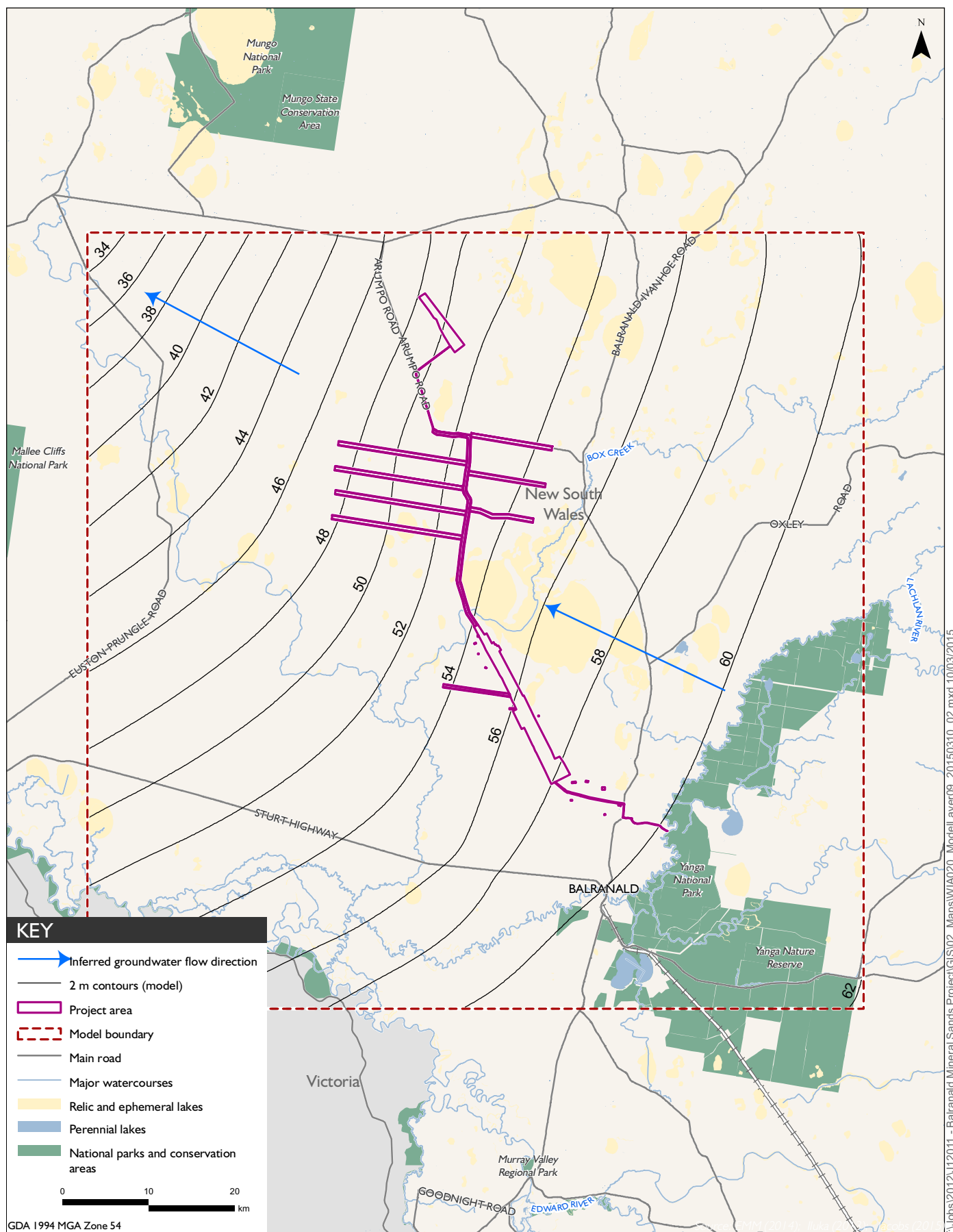
Steady state heads in model layer 9: Olney formation
