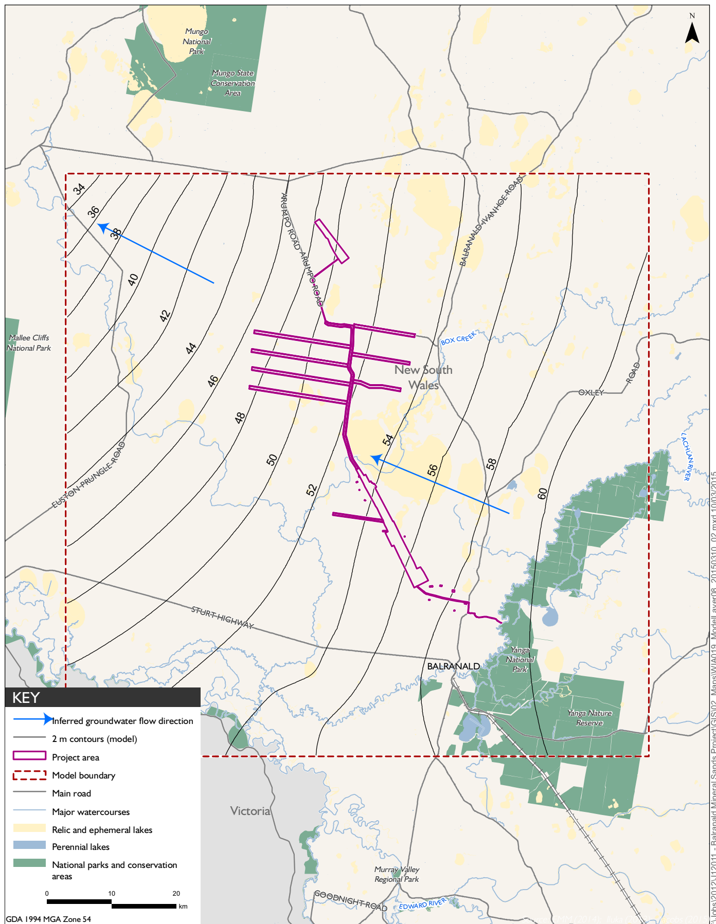
Steady state heads in model layer 8: Geera Clay
