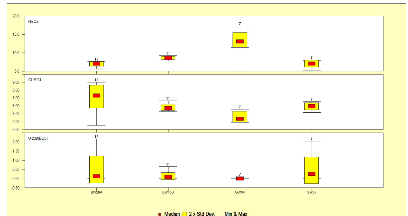
Figure 16: U-238 and ionic balance trends – cross-gradient bores (2 of 2)
