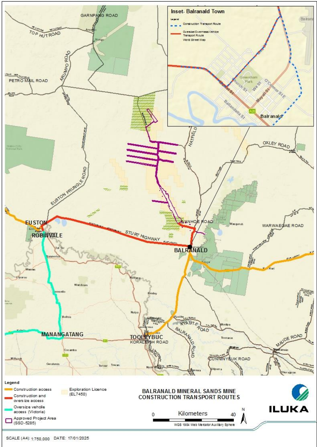
Figure 6- Construction transport routes
