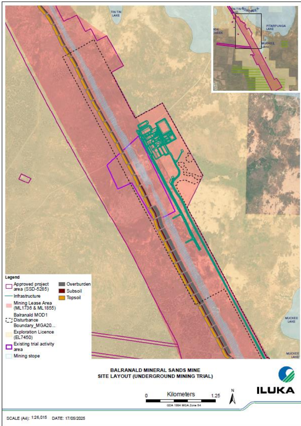
Figure 2- Site layout
