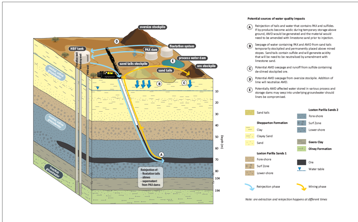
Figure 3 Mining process
