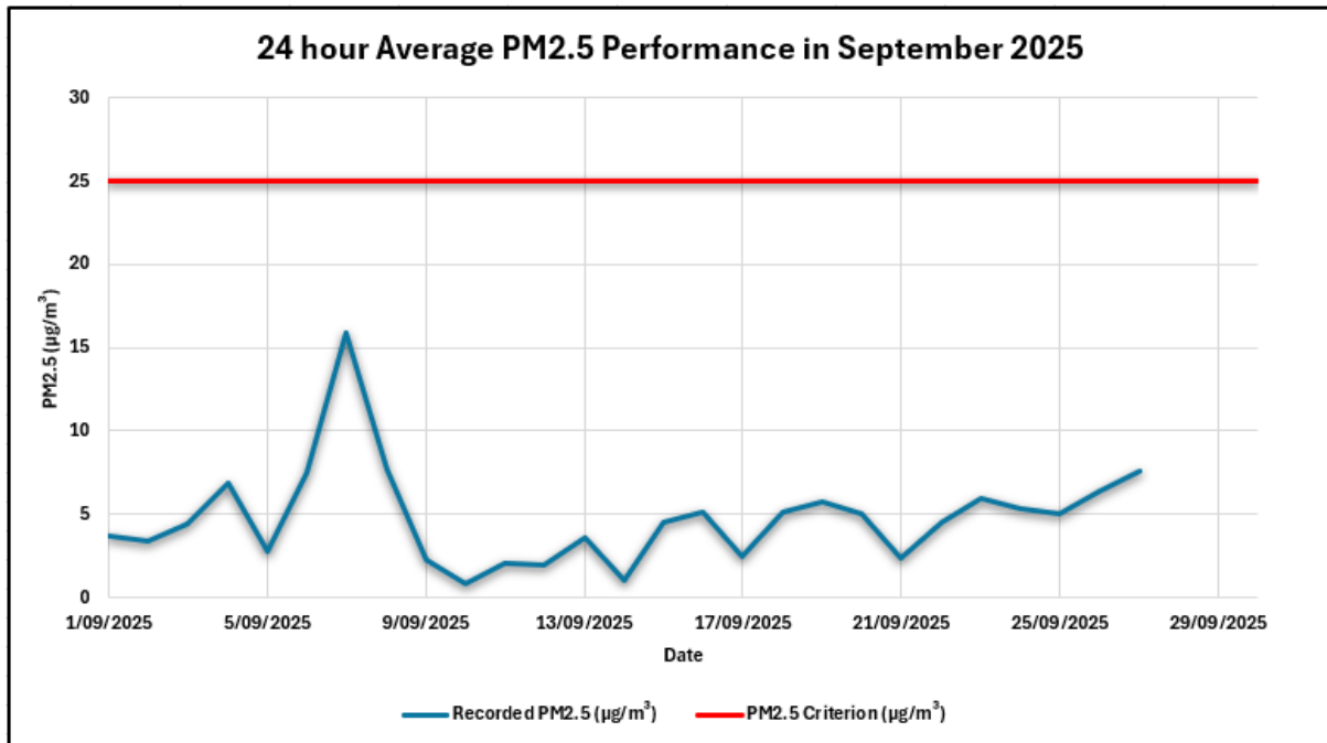
Figure 1 – 24-hour Average PM2.5 Performance in September 2025
