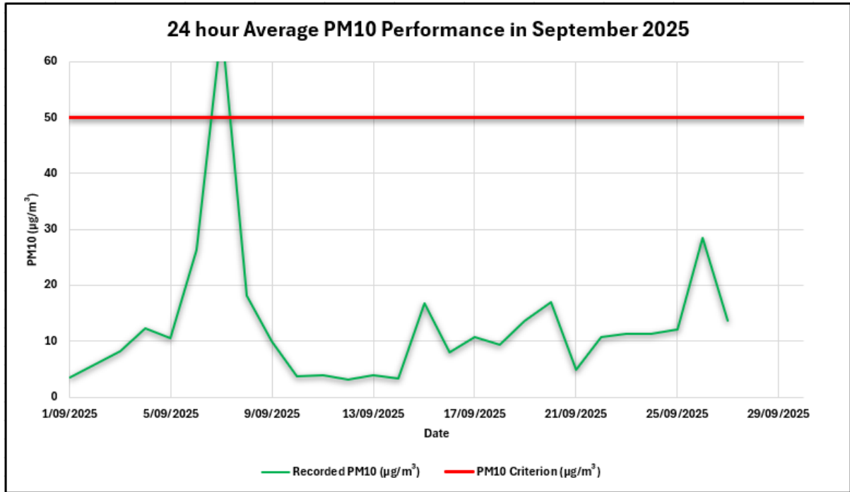
Figure 2 – 24-hour Average PM10 Performance in September 2025
